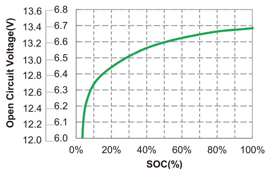
Open circuit voltage VS SOC%
