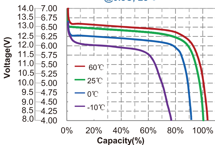
Different Temperature Discharge Curve @0.5C, 25°C
